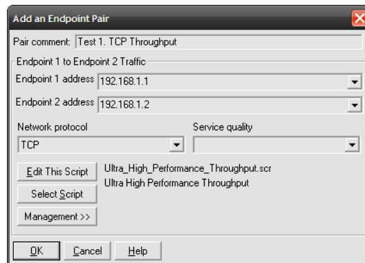
Figure 2. Pair configuration dialog for Test 1.
