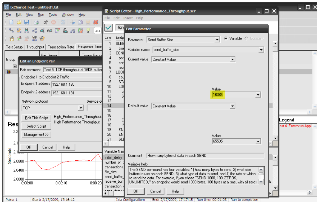
Figure 11. Adjusting the send_buffer_size to 16KB
