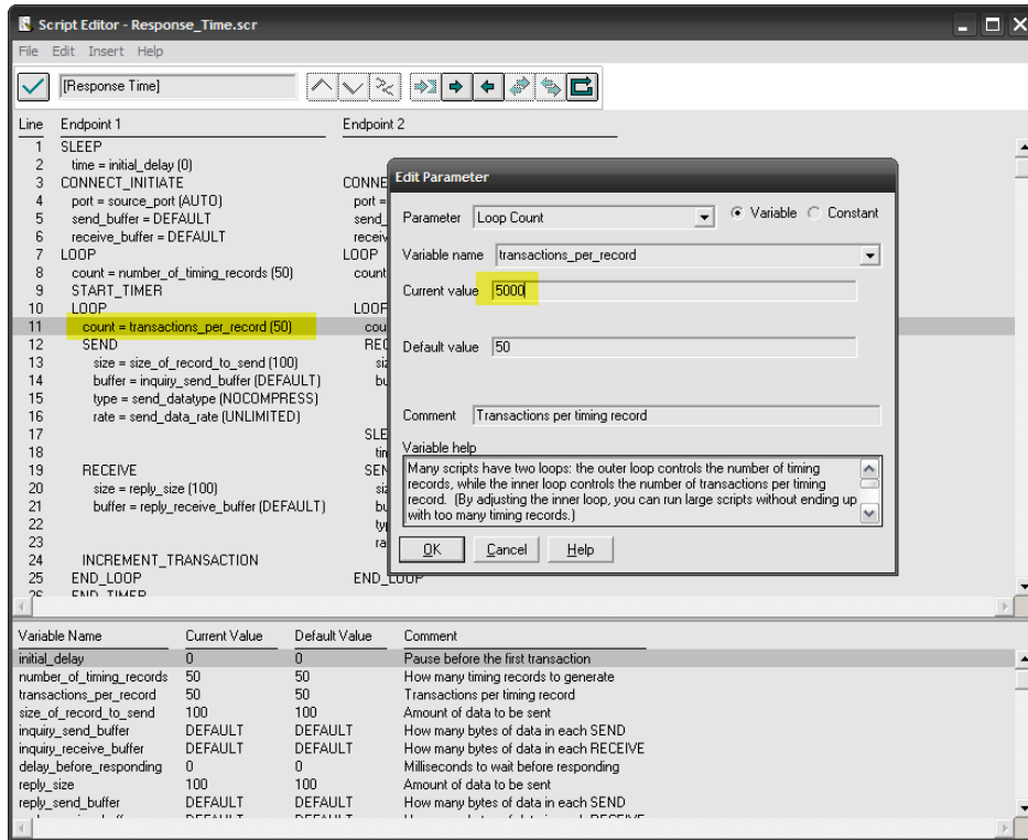
Figure 7. Changing the Loop Count variable to correct the CHR0336 warning
